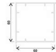
F60-ZJ, ADAPTER SQUARE POST
