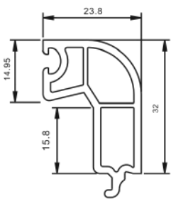
P70-KSY, SLIDING SINGLE GLASS BEAD (32*23.8)
