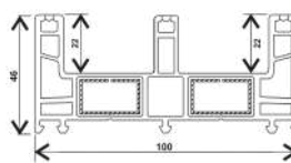
T100-K, SLIDING 3 TRACK FRAME (100*46)
