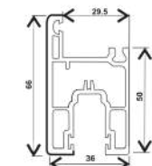
T80-DS(I), SASH SLIDING WINDOW (36*66)
