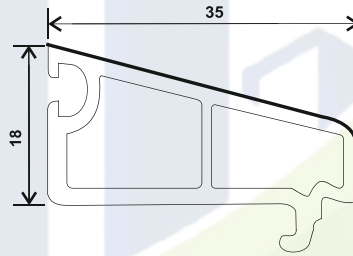
R P60-DY, BEAD CASEMENT SINGLE GLASS (18*35) 0.324
