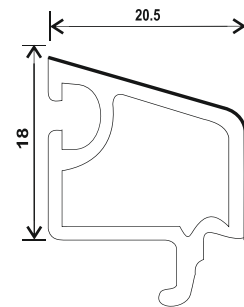
R P60-SY, BEAD DOUBLE GLASS CASEMENT (18*20.5) 0.233
