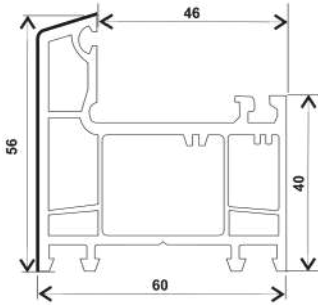
R P60 KD, FRAME CASEMENT WINDOW (60*58) 1.043
