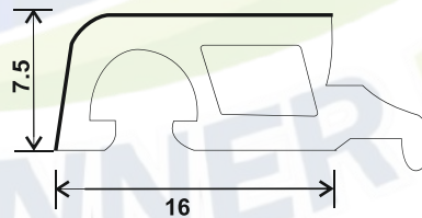
R T88-SY(I), SLIDING DOUBLE GLASS BEAD (SMALL)(16*7.5)
