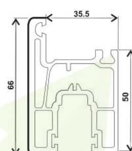
R T95-S, SASH SLIDING WINDOW (42*66) 0.956
