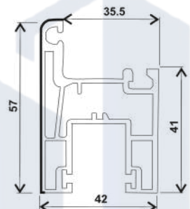
R T88-S, SASH SLIDING WINDOW (42*57) 0.847
