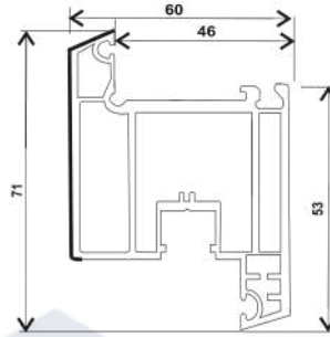
R P60 NKS, SASH WINDOW INWARD (60*71) 1.260
