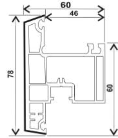
R P60-WKS, SASH WINDOW OUTWARD (60*78) 1.333
