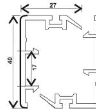
R T80-FBB(I), INTERLOCK WINDOW (27*40)
