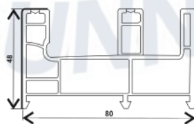
R CF-T80-PK(I), SLIDING 2.5 TRACK FRAME (80*48)
