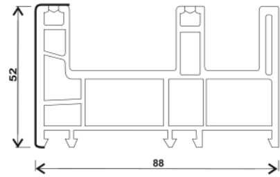
R T88-PK(J), SLIDING 2.5 TRACK FRAME (88*52) 1.322
