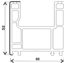
R T60-KB, SLIDING 2 TRACK FRAME (60*52) 1.025
