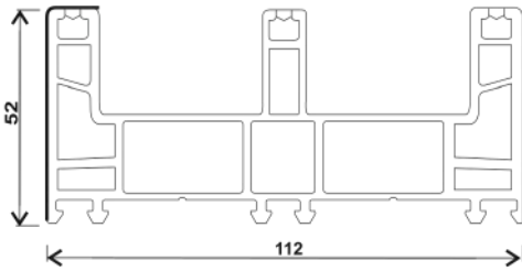
R T112-K, SLIDING 3 TRACK FRAME (112*52) 1.653
