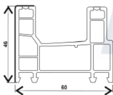
R CF-T60-LGK, SLIDING 2 TRACK FRAME (60*46)
