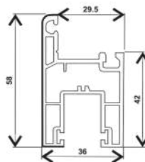
R CF-T60-S, SASH SLIDING WINDOW (36*58)
