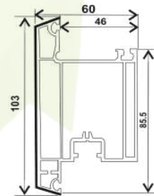
R P60-MS, SASH CASEMENT OUTWARD DOOR (60*103) 1.580
