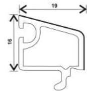
R T80-DY, SLIDING GLASS BEAD (16*19)
