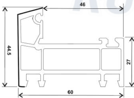
R P60-GDK, FRAME CASEMENT NARROW (60*44.5) 0.801
