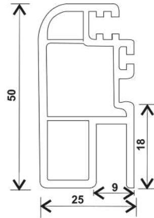
R T80-BB-DSS, SASH FLY MESH PROFILE
