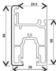
R T80-DS(I), SASH MONORAIL SLIDING (36*66)
