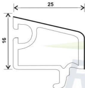
R T88-DY, SLIDING SINGLE GLASS BEAD (16*25) 0.269
