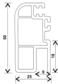
T80-88-DSS, SASH FLY MESH PROFILE
