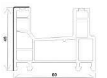
CF-T60-LGK, SLIDING 2 TRACK FRAME (60*46)
