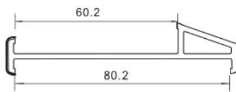
F60-80-PB, COUPLING 2.5 TRACK ECO
