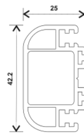
T80-88-SST, MULLION FLY SASH
