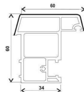
P60-FZT(II)-D, MULLION CASEMENT MOVABLE (60*60)
