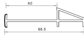
6F60-80-PB, COUPLING 2.5 TRACK
