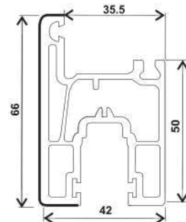
T95-S, SASH SLIDING WINDOW (42*66)
