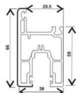
T80-DS(I), SASH SLIDING WINDOW (36*66)
