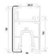
T80-DS(I), SASH MONORAIL SLIDING (36*66)
