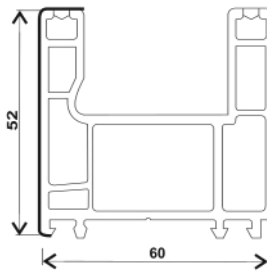
T60-KB, SLIDING 2 TRACK FRAME (60*52)
