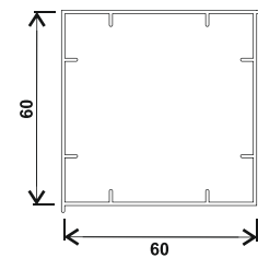
F60-ZJ, ADAPTER SQUARE POST
