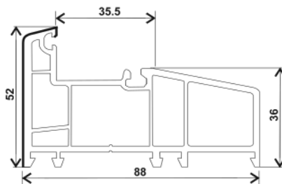
T88-GDK(B2), SLIDING 2.5 TRACK FIXED FRAME
