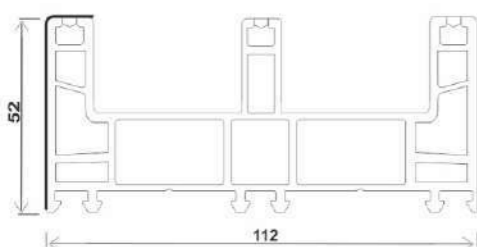
T112-K, SLIDING 3 TRACK FRAME (112*52)
