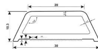
G-B GEORGIAN BAR
