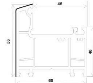
P60 KD, FRAME CASEMENT WINDOW (60*58)
