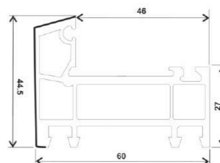
P60-GDK, FRAME CASEMENT NARROW (60*44.5)
