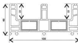
T100-K, SLIDING 3 TRACK FRAME (100*46)
