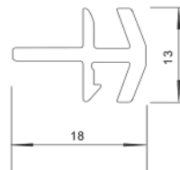
F-GMT, COUPLING SMALL ONE SIDED
