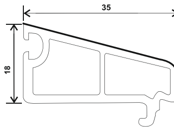
P60-DY, BEAD CASEMENT SINGLE GLASS (18*35)
