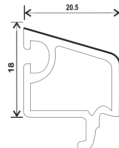
P60-SY, BEAD DOUBLE GLASS CASEMENT (18*20.5)
