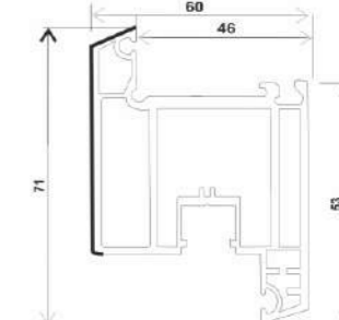
P60 NKS, SASH WINDOW INWARD (60*71)
