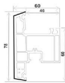
P60-WKS, SASH WINDOW OUTWARD (60*78)
