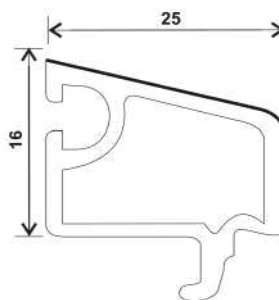
T88-DY, SLIDING SINGLE GLASS BEAD (16*25)
