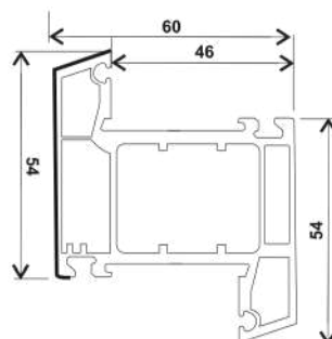
P60-ZZT(B), MULLION CASEMENT Z
