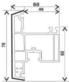
P60-WKS, SASH WINDOW OUTWARD (60*78)
