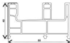
CF-T80-PK(I), SLIDING 2.5 TRACK FRAME (80*48)
