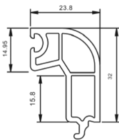
P70-KSY, SLIDING SINGLE GLASS BEAD (32*23.8)
