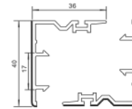
T80-DFB, INTERLOCK WINDOW (36*40)
