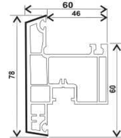
R P60-WKS, SASH WINDOW OUTWARD (60*78) 1.333
