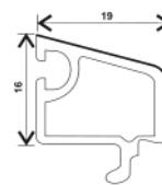
T80-DY, SLIDING SINGLE GLASS BEAD (16*19)
