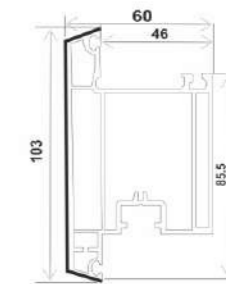
P60-MS, SASH CASEMENT OUTWARD DOOR (60*103)
