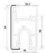
T80-DS(II), SASH SLIDING WINDOW (36*66)
