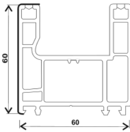
T60-K, SLIDING 2 TRACK FRAME (60*60)
