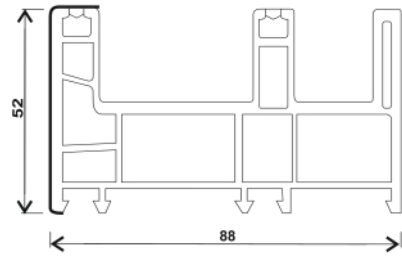
T88-PK(J), SLIDING 2.5 TRACK FRAME (88*52)
