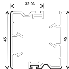
T95-FB, INTERLOCK WINDOW SASH (32.03*45)
