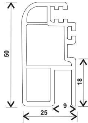
R T80-BB-DSS, SASH FLY MESH PROFILE
