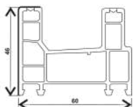
CF-T60-LGK, SLIDING 2 TRACK FRAME (60*46)
