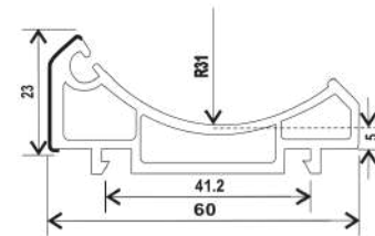
F-WXZJ, ADAPTOR BAY POST 62MM
