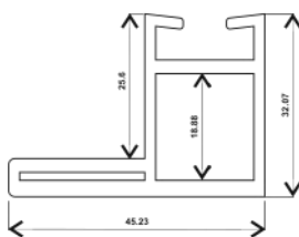
F-SSG ADDON FRAME
