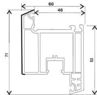
P60 NKS, SASH WINDOW INWARD (60*71)
