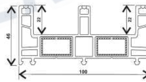
R T100-K, SLIDING 3 TRACK FRAME (100*48)
