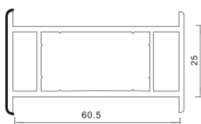
F60-PG, COUPLING BIG
