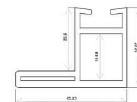
F-SSG ADDON FRAME
