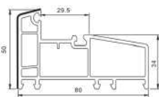
T80-GDK, SLIDING 2.5 TRACK FIXED FRAME
