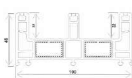
T100-K, SLIDING 3 TRACK FRAME (100*46)
