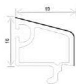
T80-DY, SLIDING SINGLE GLASS BEAD (16*19)
