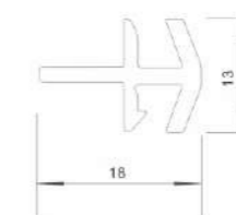
F-GMT, COUPLING SMALL ONE SIDED
