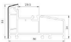
T80-GDK, SLIDING 2.5 TRACK FIXED FRAME
